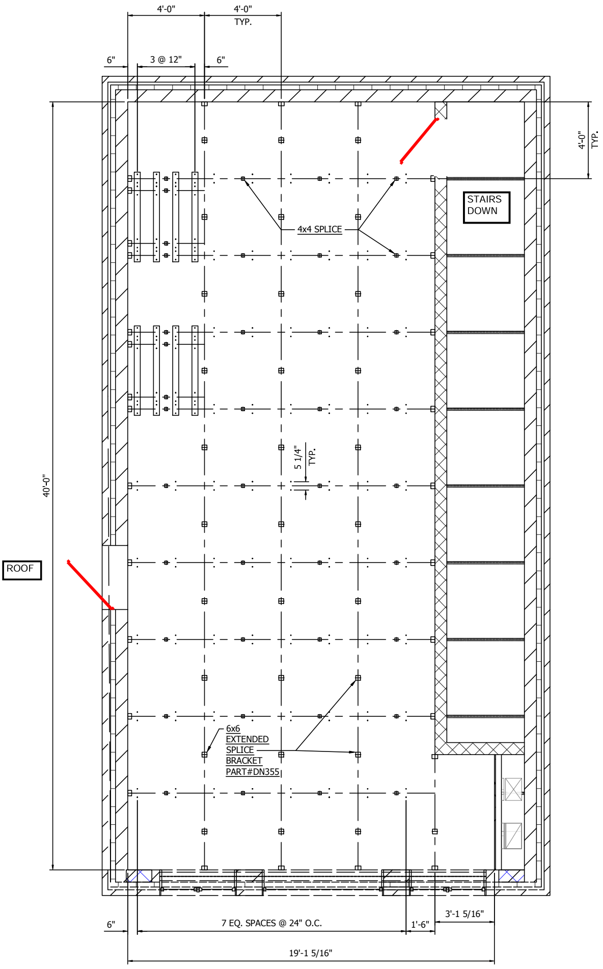
1 LEVEL 2 - BDLG B HANGER ROD LAYOUT
